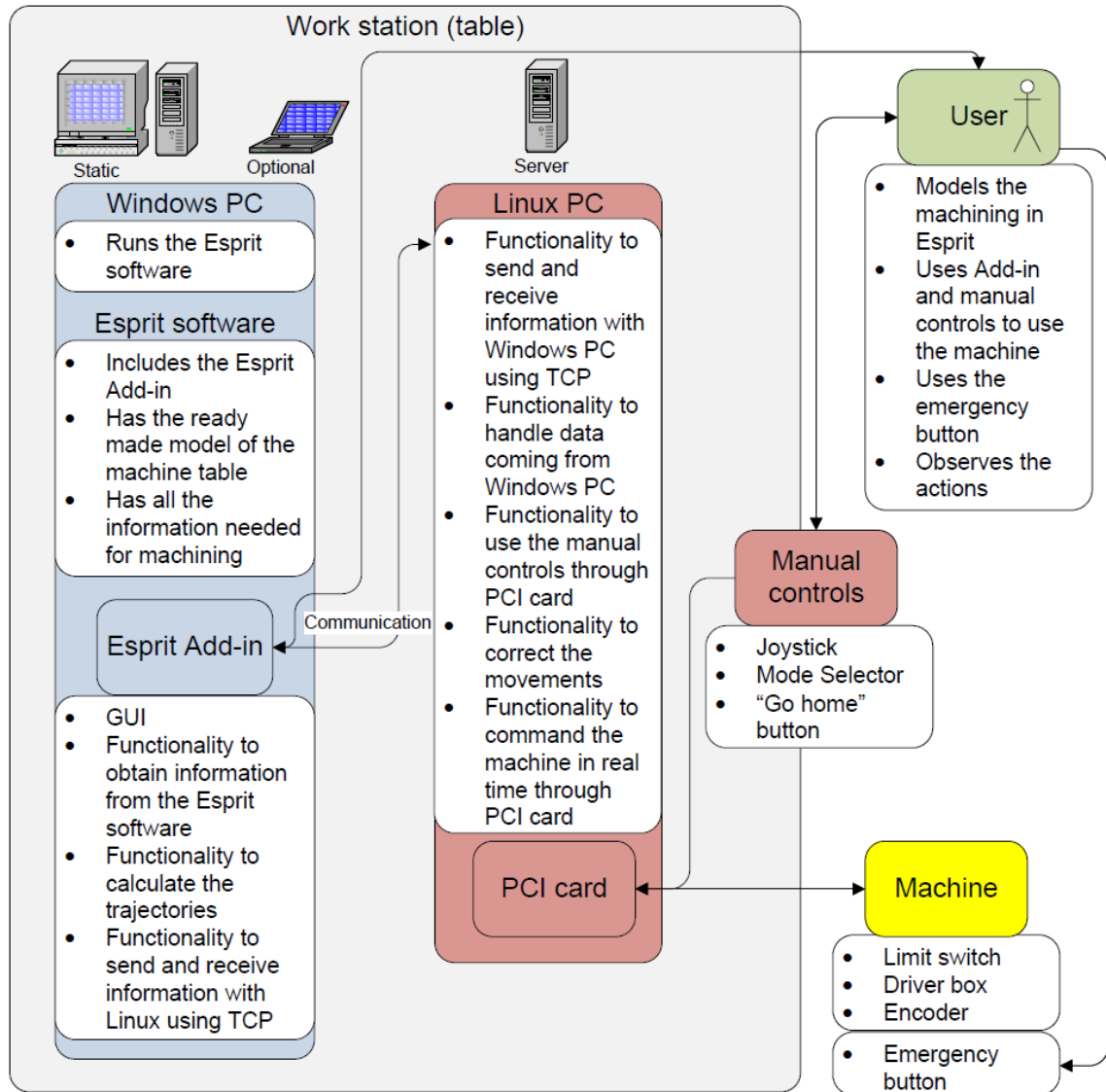
Figure 1 : Machine architecture
