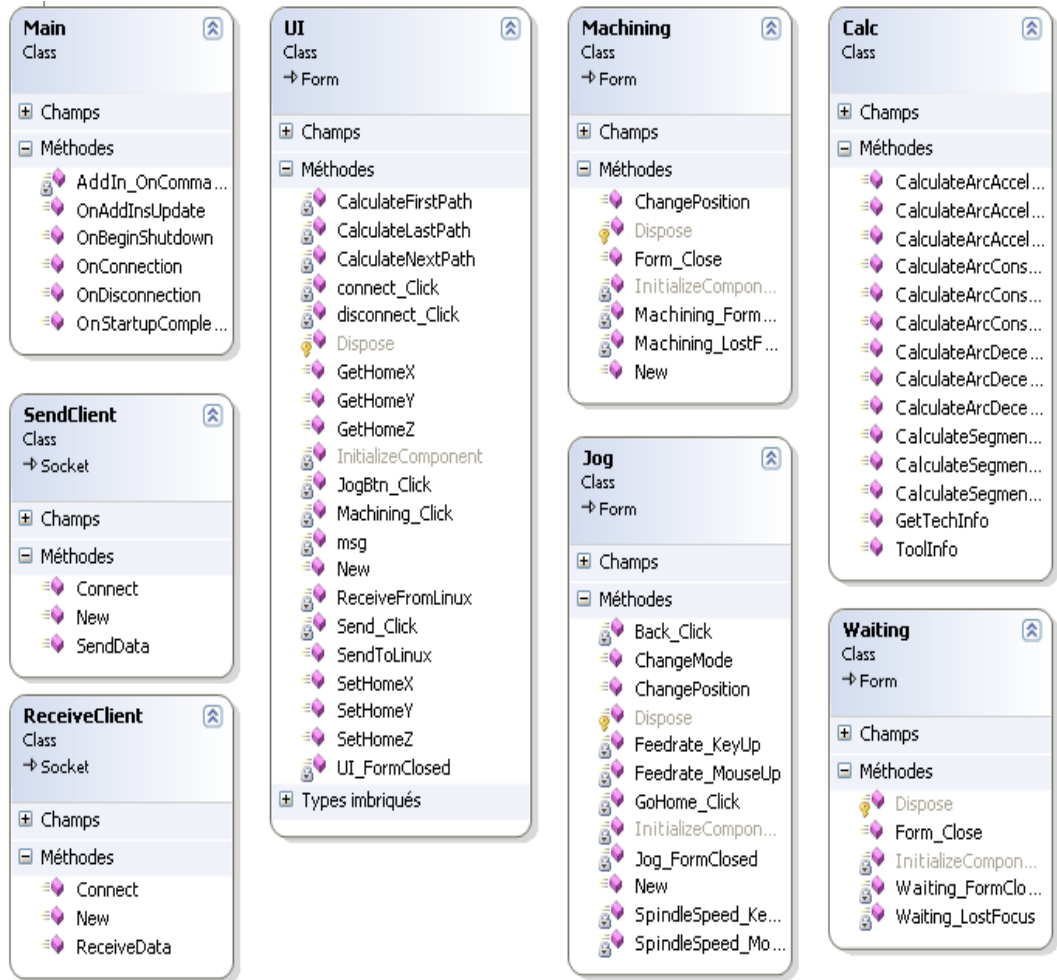
Figure 3 : AddIn composition
