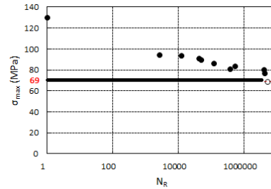
Figure 5. [+45/-45/+45/-45] s experimental Wöhler curve for ( \sigma_{xx} = 50 MPa) and limit of fatigue from self-heating tests
