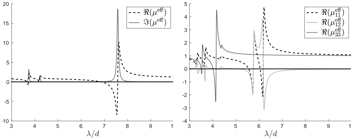
FIGURE 2. Tensor \boldsymbol{\mu}^{\text{eff}} as a function of \lambda/d for \varepsilon_r = 100 + i . On the left \Sigma = \Sigma_1 is a cube of size 0.6 and tensor \boldsymbol{\mu}^{\text{eff}} is scalar; on the right \Sigma = \Sigma_2 is a L-shape inclusion (and \boldsymbol{\mu}_{22}^{\text{eff}} = \boldsymbol{\mu}_{11}^{\text{eff}}, \boldsymbol{\mu}_{13}^{\text{eff}} = \boldsymbol{\mu}_{23}^{\text{eff}} = 0 ).
