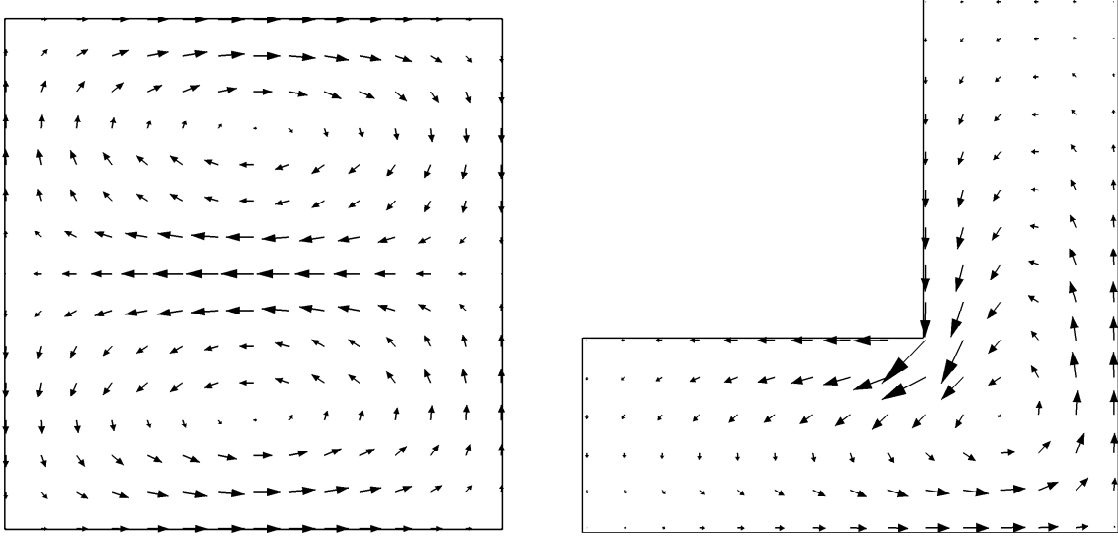
FIGURE 4. Left side: horizontal section of eigenvector \mathbf{f}_4 in the cubic geometry (mode that is not excited). Right side: horizontal section of field \mathbf{J}^3 for \lambda/d = 4.17 in the L-shape geometry.
