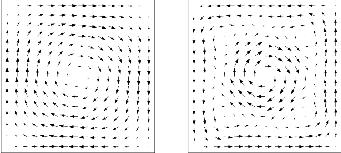
FIGURE 3. Horizontal section of \mathbf{J}^3 for the cubic geometry. Left side: \lambda/d = 7.5 (fundamental resonance). Right side: \lambda/d = 3.76 . (resonance associated with the 24th eigenvalue).
