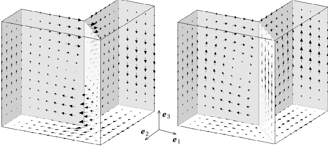
FIGURE 5. Representation of field J^1 in the case of a L-shape inclusion \Sigma . On the left, \lambda/d = 6.2 (first mode is excited) and on the Right \lambda/d = 5.7 (second mode is excited)
