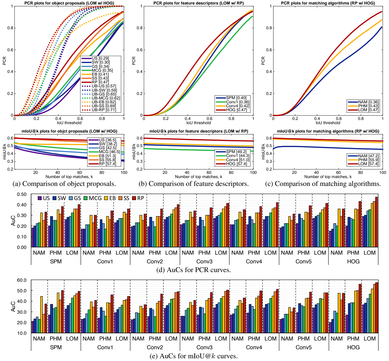
Figure 5. RSF benchmark evaluation on (a-c) region matching precision (top, PCR plots) and match retrieval accuracy (bottom, mIoU@k plots), and (d-e) AuCs for different combinations of object proposals, features, and matching algorithms: (a) Evaluation for LOM with HOG [11], (b) evaluation for LOM with RP [40], (c) evaluation for RP with HOG [11], (d) AuCs for PCR curves, and (e) AuCs for mIoU@k curves. The AuC is shown in the legend. (Best viewed in color.)
