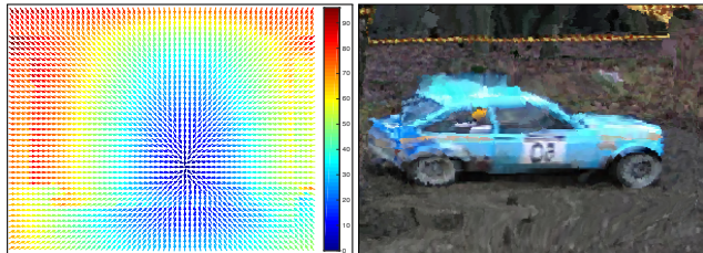
(b) Match visualization.
