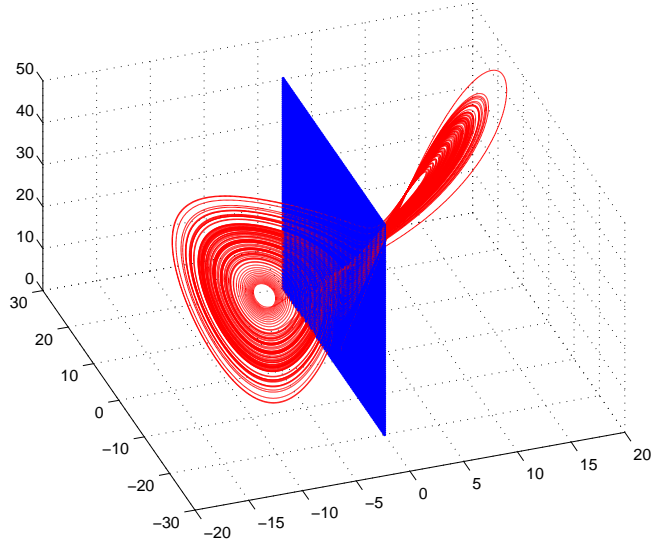
Figure 1: Lorenz attractor and the map \mathcal{S}_3
