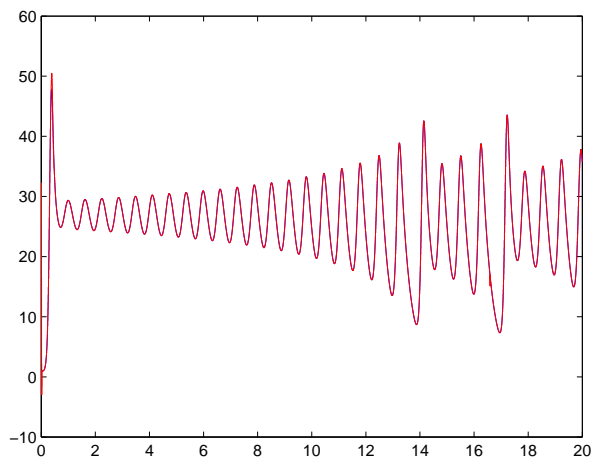
Figure 3: The stat x_3 and its estimate \hat{x}_3
