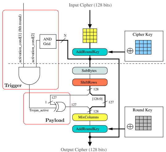
Fig. 2: Trojan inserted on AES 128 bits
