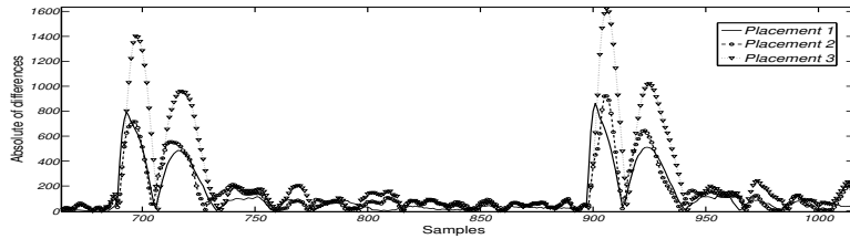
Fig. 7: Impact on EM measurement for different locations of Trojan 1.7% on FPGA Virtex 5
