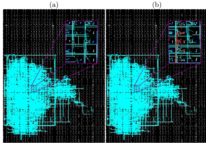
Fig. 3: Placement and routing of circuits on FPGA Virtex 5. for (a) AES 128 bit without HT and (b) AES 128 bit with HT 1.7%
