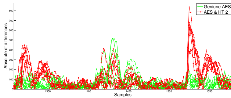
Fig. 4: Impact of Process Variations on EM measurements
