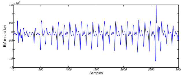
Fig. 5: EM Measurement for single encryption.
