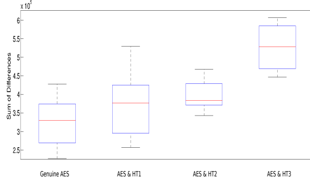
Fig. 6: Sum of absolute differences (SoD) Dg and Dt for the four implementations
