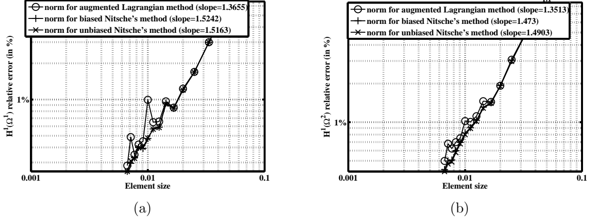
Figure 14: Comparison of convergence curves in 2D frictionless case for the method \theta = -1 , with \gamma_0 = 1/100 and P_2 finite elements for the relative H^1 -norm of the error on \Omega^1 (a) and on \Omega^2 (b) for different formulations of contact.
