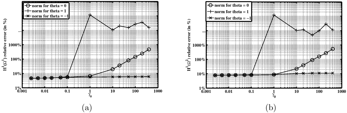
Figure 15: Influence of \gamma_0 on the H^1 -norm error for different values of \theta in the 2D frictionless case and with P_2 finite elements on \Omega^1 (a) and on \Omega^2 (b).
