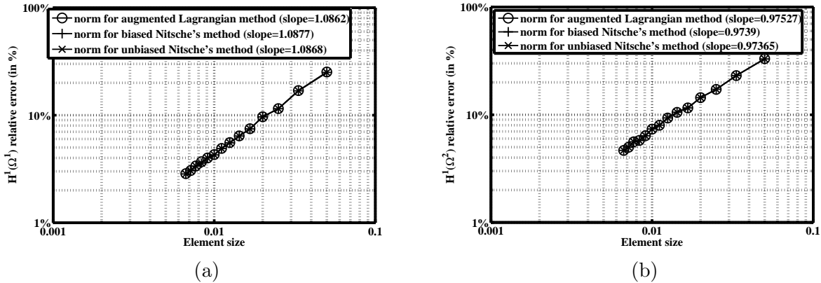
Figure 13: Comparison of convergence curves in 2D frictionless case for the method \theta = -1 , with \gamma_0 = 1/100 and P_1 finite elements for the relative H^1 -norm of the error on \Omega^1 (a) and on \Omega^2 (b) for different formulations of contact.
