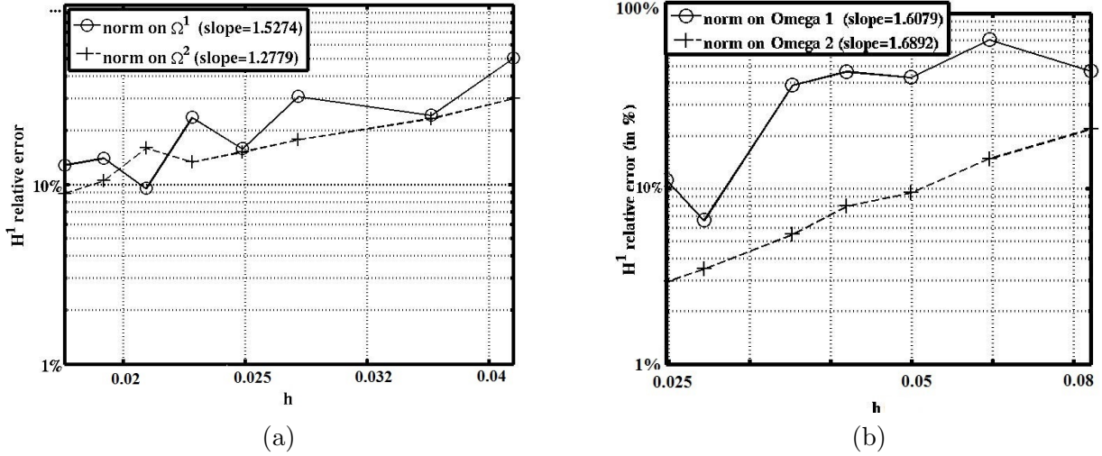
Figure 12: Convergence curves in 3D for the method \theta = -1 , with \gamma_0 = 1/100 for the relative H^1 -norm of the error with P_1 finite elements (a) and P_2 finite elements (b).
