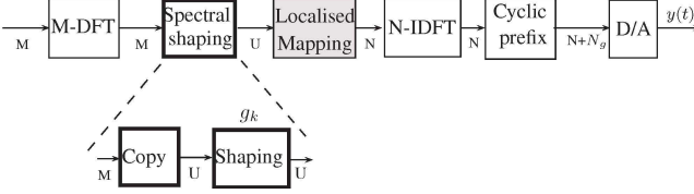
Fig. 2. LFDMA with spectral shaping M \leq U \leq 2M
