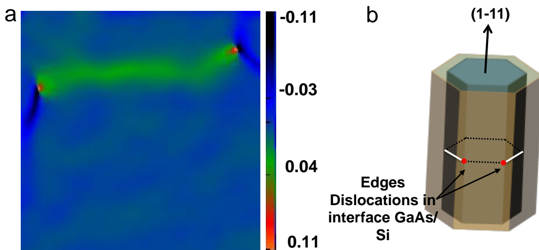
Figure 5. (a) Strain field map, where a tensile region crossing the nanowire diameter is visible (green line) and (b) Sketch of the nanowire assuming an edge dislocation loop , lying in a (1 \bar{1} 1) plane at the core–shell interface with Burgers vector b= a/3[1\bar{1}1] .
