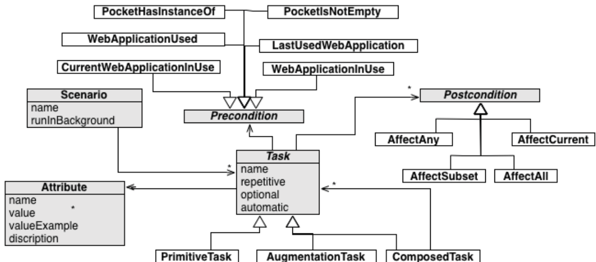
Fig. 4. The DSL metamodel
