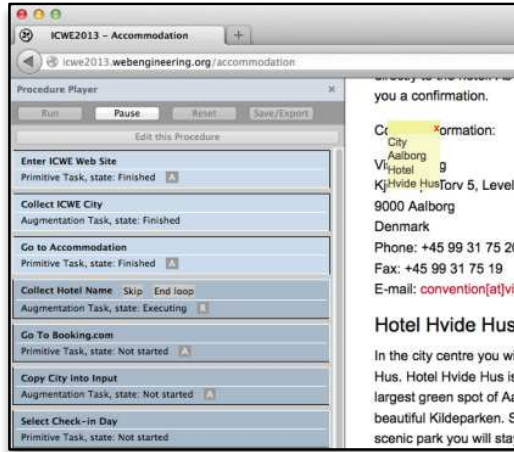
Fig. 6.a. Task Execution: collecting accommodation
