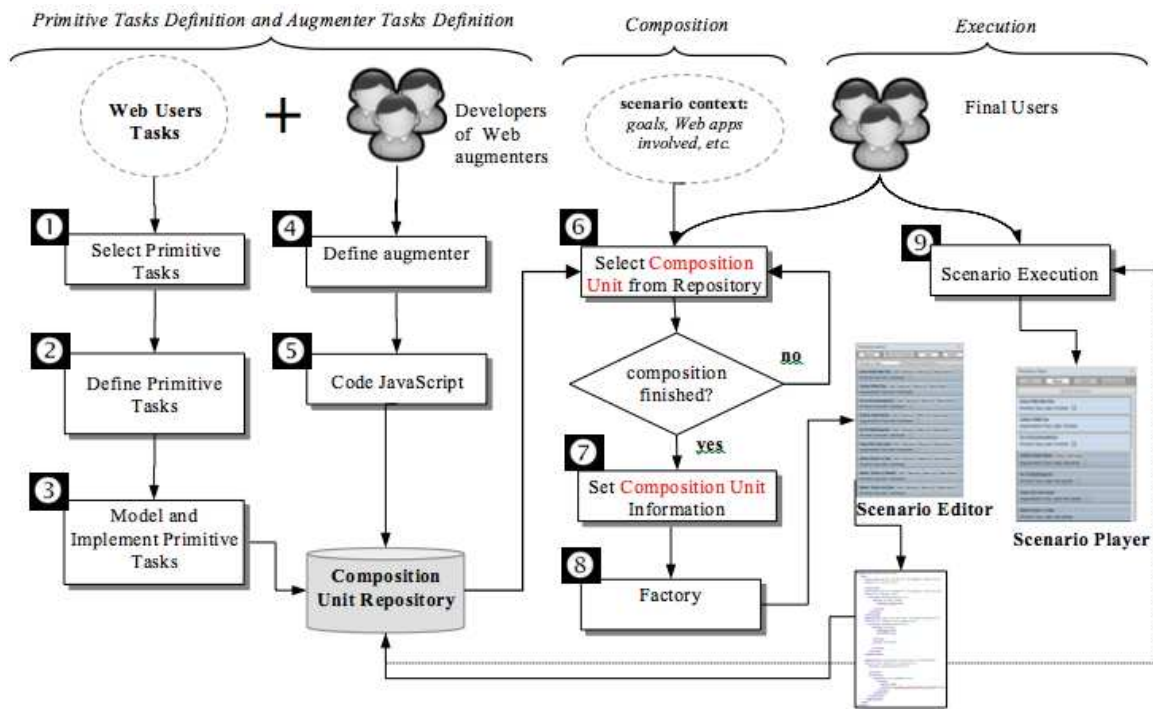
Fig. 3. Overview of the approach
