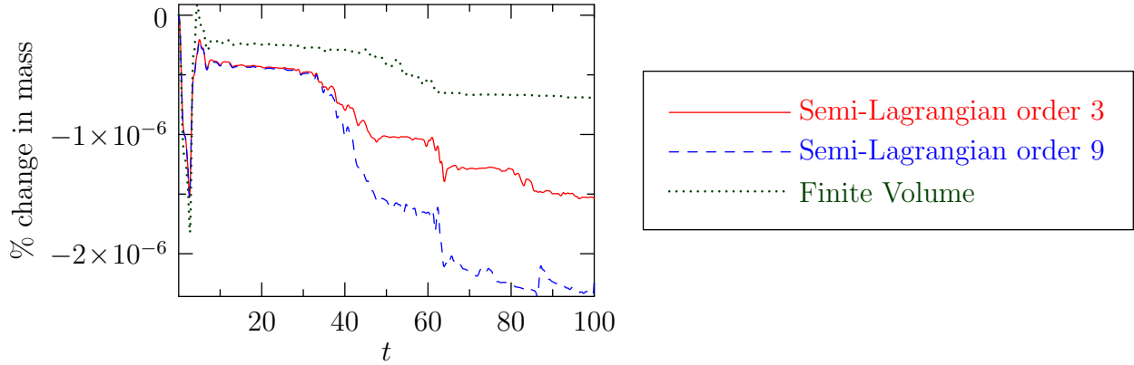
FIGURE 7. Time evolution of the change in mass as function of time for the strong Landau damping 1D test case. The semi-Lagrangian schemes (order 3: cubic spline interpolation, order 9: Lagrange interpolation) and the finite volume scheme ( \varepsilon = 0.02 ) are compared.
