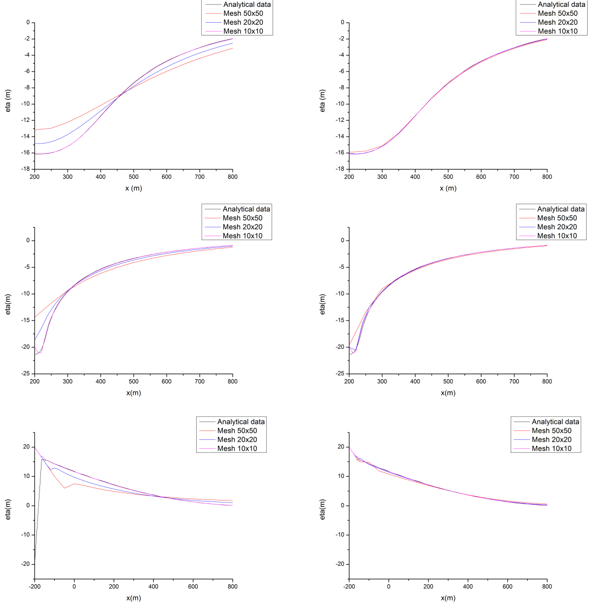
Figure 4. Free surface at t = 160 (top), t = 175 (middle) e t = 220 seconds (bottom) for the run-up on linear ramp. the left panel corresponds to the first-order scheme and the right panel to the second-order scheme.
