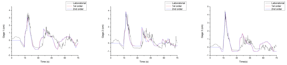
Figure 8. Comparison of laboratorial and numerical data, for three tide gauges located at points (4.521, 1.196) (tide gage 1), 4.521, 1.696 (tide gage 2) and 4.521, 2.196 (tide gage 3).
