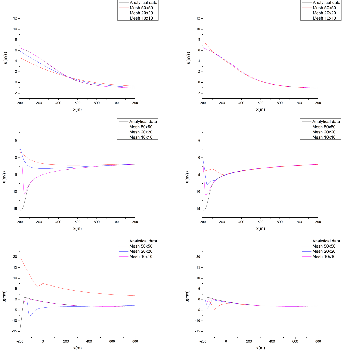
Figure 5. Water velocity at t = 160 (top), t = 175 (middle) e t = 220 seconds (bottom) for the run-up on linear ramp. the left panel corresponds to the first-order scheme and the right panel to the second-order scheme.
