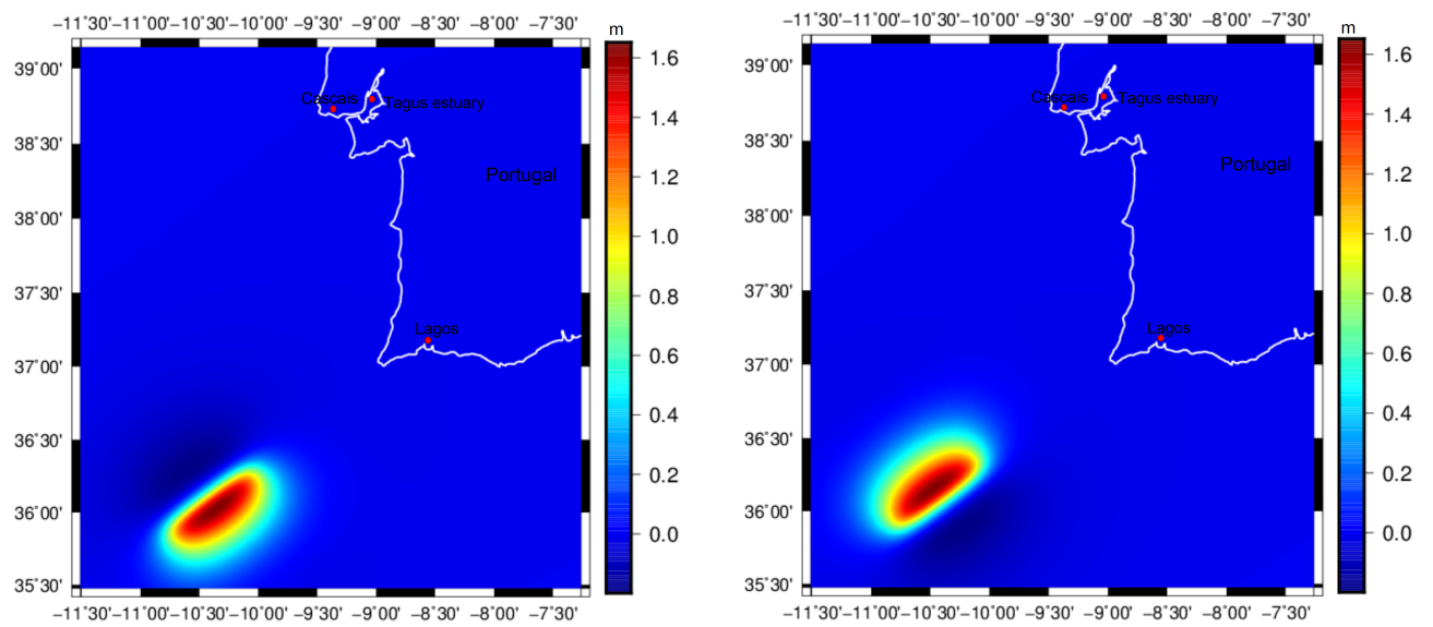
Figure 10. Initial deformation, considering a NE-SW (left) and SW-NE (right) fault orientation. Location of the simulation PoI's.
