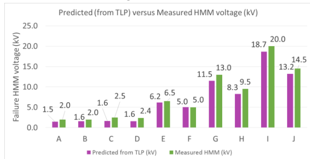
Figure 32: Comparison of predicted & actual HMM failure charging voltage
