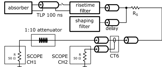
Figure 18: 50Ω load setup
