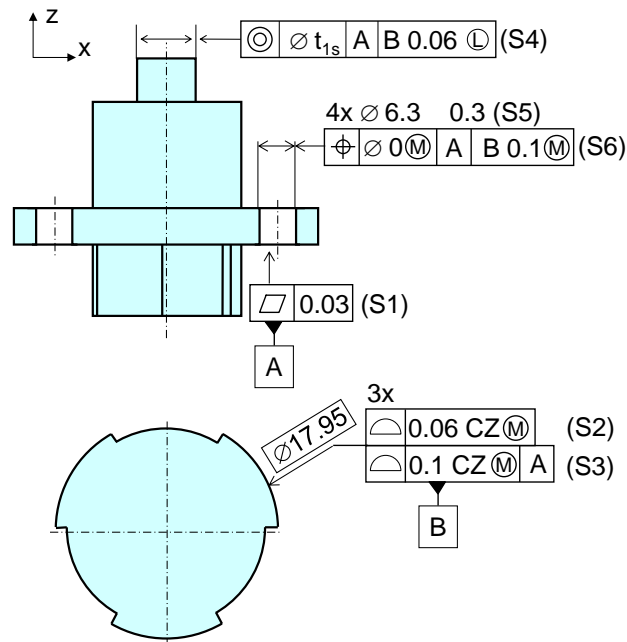
Figure 14: Tolerancing considering B as complex surface
