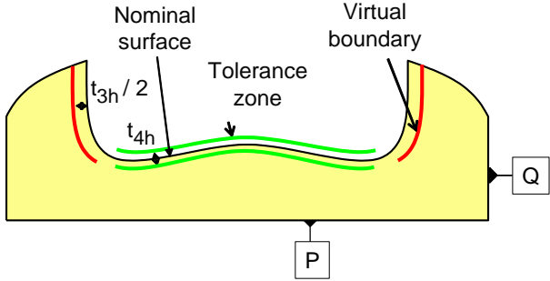
Figure 30: Specification of the housing.
