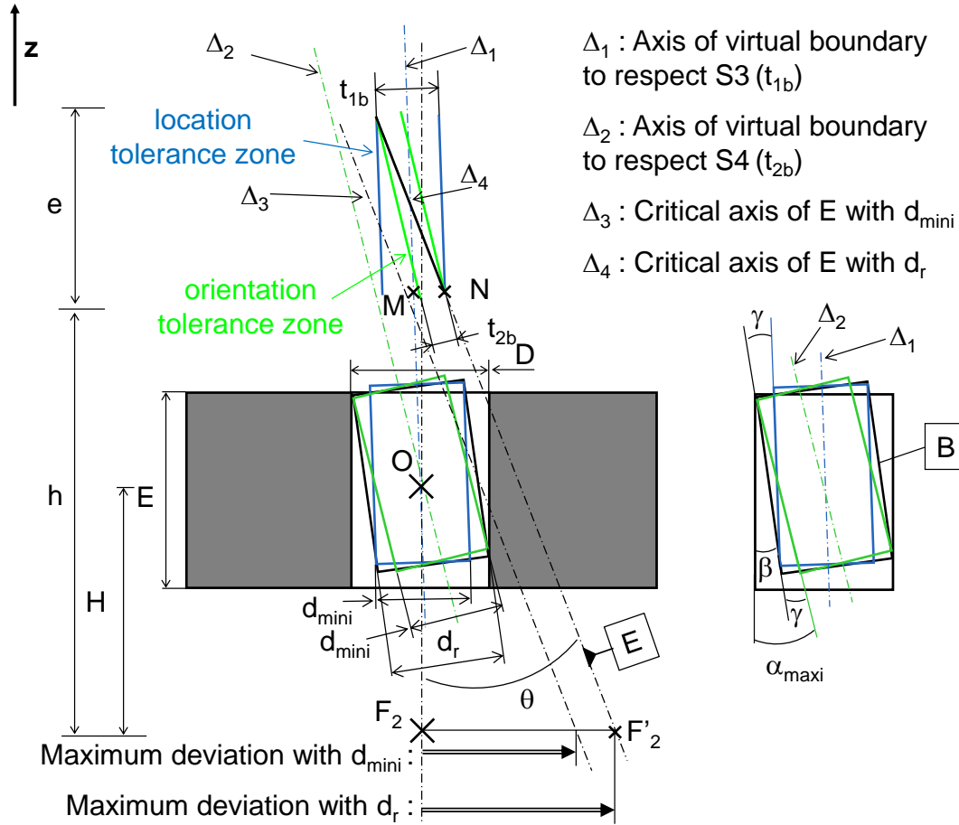
Figure 8: Three-dimensional model for displacement of F2 in general case
