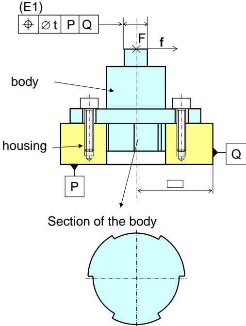
Figure 10: Secondary feature composed of several cylindrical sectors
