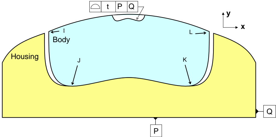
Figure 21: hybrid prismatic link
