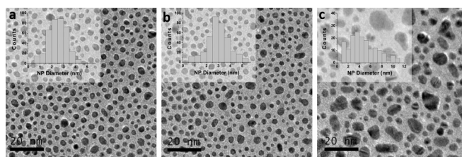
FIG. 1. TEM images of CoPt NPs with the corresponding particle size distribution in the insets. (a) As-grown NPs (sample A), (b) NPs after 1 h at 650 °C (sample B), and (c) NPs after 1 h at 750 °C (sample C).
