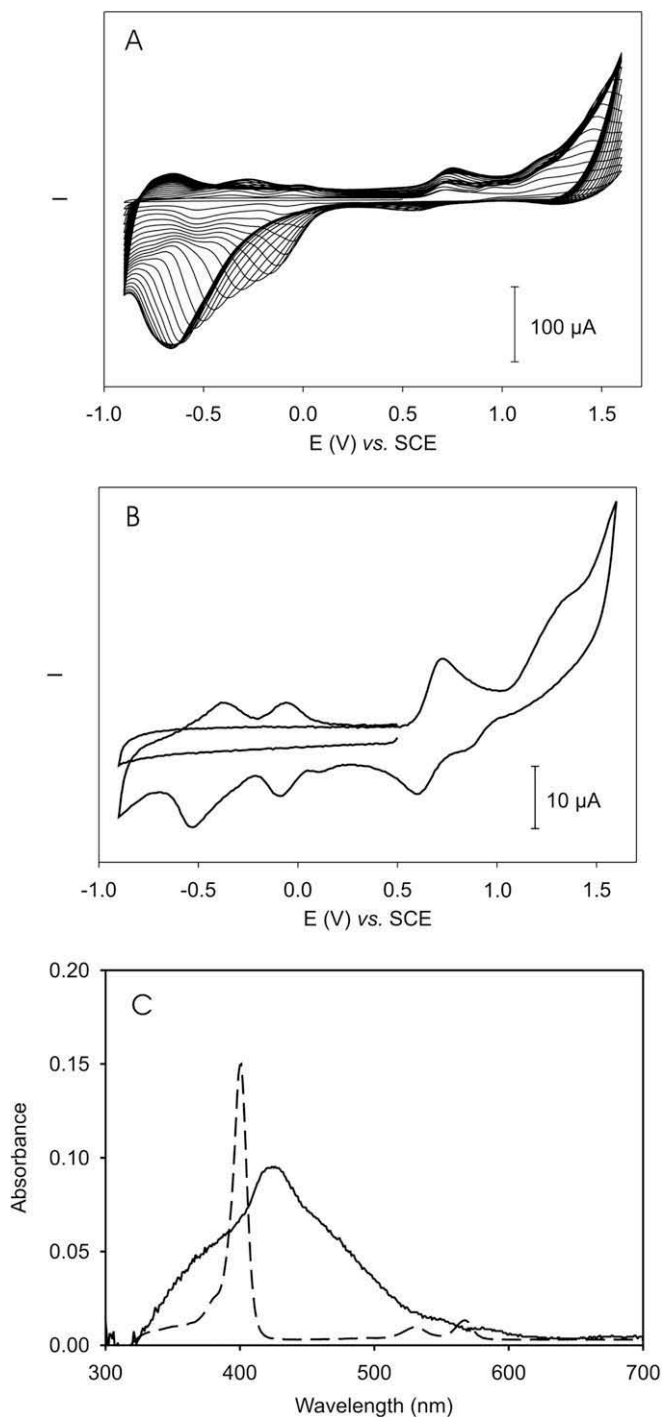
Fig. 3. (A) Cyclic voltammograms recorded during electropolymerization of ZnOEP with tbpe . Working electrode: ITO. (B) The first scan recorded during electropolymerization. (C) UV-vis spectra; dotted line: ZnOEP in \text{CH}_2\text{Cl}_2 ; full line: poly-ZnOEP-tbpe .
