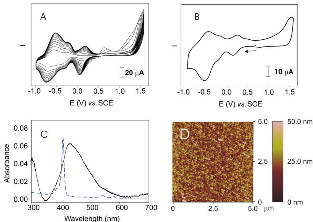
Fig. 2. (A) Cyclic voltammograms recorded during electropolymerization of MgOEP with 4,4'-bipyridine. Working electrode: ITO. (B–D) The modified ITO electrode with poly-MgOEP obtained after 25 iterative scans in the presence of 4,4'-bipyridine. (B) Cyclic voltammogram. (C) UV-vis spectrum (dotted line: MgOEP in \text{CH}_2\text{Cl}_2 ). (D) Atomic force micrograph (AFM).
