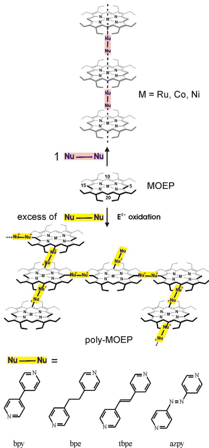
Fig. 1. Top: proposed structure of the octaethylporphyrin coordination polymers where M = Ru, Co, Ni. Bottom: polymerization scheme of MOEP (M = H 2 , Co II , Mg II , Ni II , Ru II (CO), Zn II ) and Lewis bases Nu–Nu used for the electropolymerizations. Nu–Nu = 4,4'-bipyridine (bpy), trans-1,2-bis(4-pyridyl)ethane (tbpe), 1,2-bis(4-pyridyl)ethane (bpe), 4,4'-azopyridine (azpy). For clarification, the coordination of Nu–Nu has been omitted.
