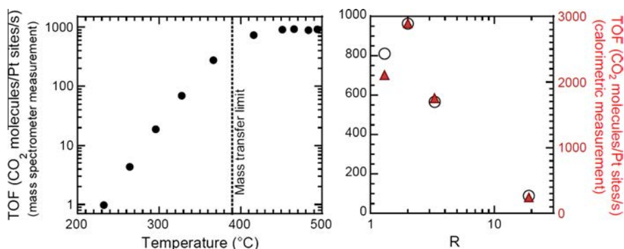
Fig. 2. Measured turnover frequencies (TOFs) for 200 mbar of total pressure of \text{CO} + \text{O}_2 . Left panel. TOF as a function of the temperature of the Pt sample for a fixed stoichiometric proportion R = P_{\text{CO}}/P_{\text{O}_2} = 2/1 . Right panel. TOFs for different stoichiometries from \text{O}_2 rich ( R = 1.5 ) to \text{CO} rich ( R = 19 ) gas mixtures for T \approx 490^\circ\text{C} . TOFs are either derived from mass spectrometer (black symbols, left vertical axis) or from calorimetric measurements (red symbols, right vertical axis). (For interpretation of the references to color in this figure legend, the reader is referred to the web version of this article.)
