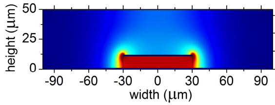
Figure S2. Modal profile at 12GHz of a 60 \mu\text{m} wide metal-metal QCL operating at a center frequency of 2.7THz.
