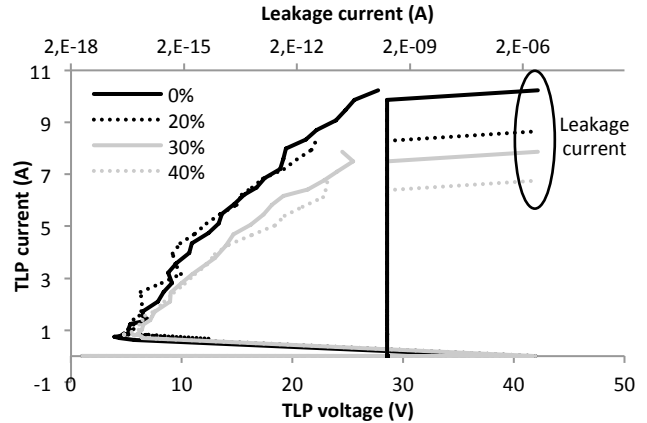
Fig. 6: Effect of channel reduction from 0 to 40 % to the TLP characteristics of the 3P1N (75% IGBT) structure.
