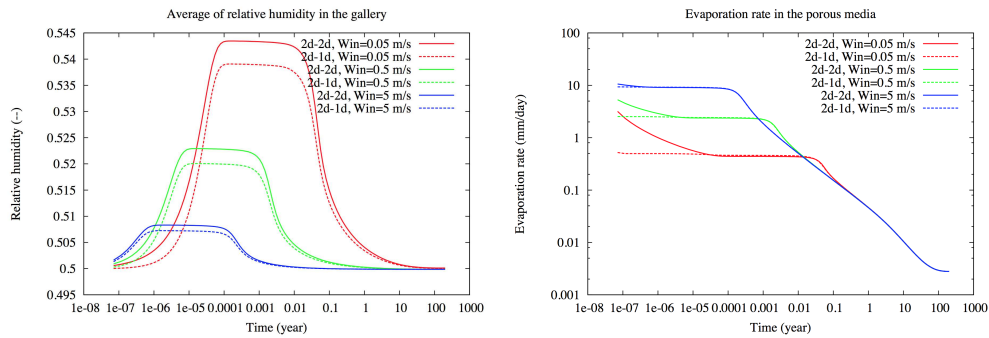
Figure 8: Comparison of the solutions obtained by the 2D-2D and 2D-1D models with L = 100 m and the mesh 100 \times 200 : average of the relative humidity in the gallery (left), evaporation rate at the interface (right) as a function of time.
