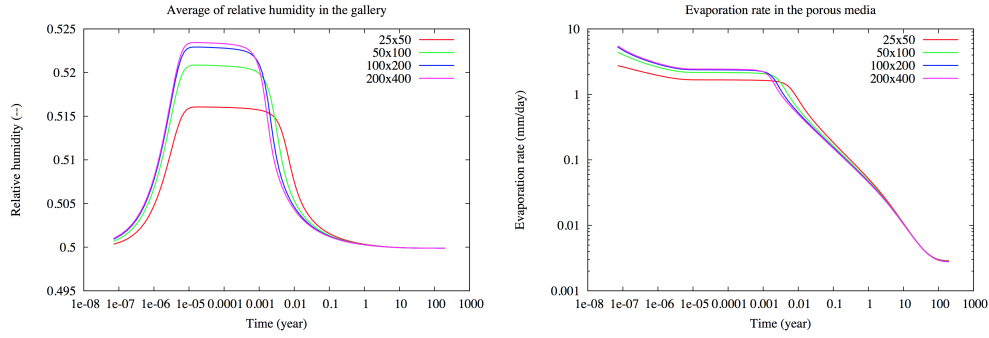
Figure 6: For each mesh and for L = 100 m, w_{in} = 0.5 \text{ m}\cdot\text{s}^{-1} : average of the relative humidity in the gallery (left) and evaporation rate at the interface (right) as a function of time.
