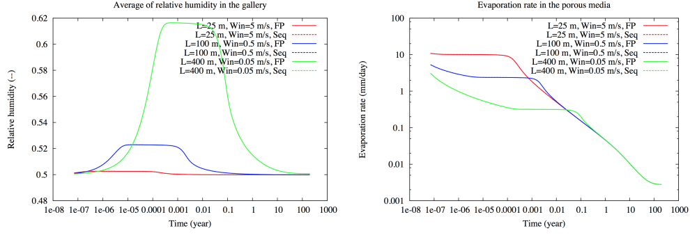
Figure 9: Comparison of the solutions obtained by the fixed-point (FP) and sequential (Seq) algorithms with the mesh 100 \times 200 : average of the relative humidity in the gallery (left), evaporation rate at the interface (right) as a function of time.
