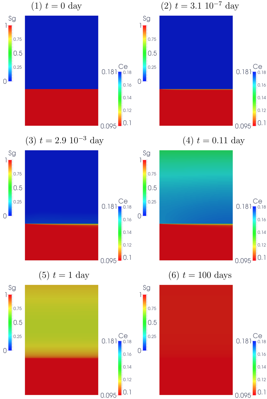
Figure 17: Gas saturation in the porous medium and water molar fraction in the gallery with w_{in} = 10 \text{ m.s}^{-1} and the mesh 100 \times 283 at (1) t = 0 day, (2) t = 3.1 \cdot 10^{-7} day, (3) t = 2.9 \cdot 10^{-3} day, (4) t = 0.11 day, (5) t = 1 day, (6) t = 100 days.
