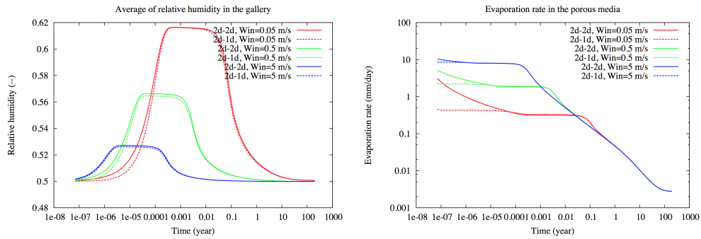
Figure 8: Comparison of the solutions obtained by the 2d-2d and 2d-1d models with L = 400 m and the mesh 100 \times 200 : average of the relative humidity in the gallery (left), evaporation rate at the interface (right) as a function of time.
