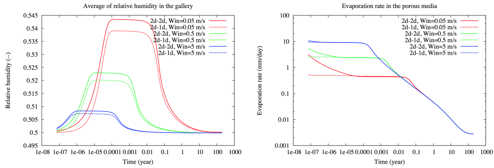
Figure 7: Comparison of the solutions obtained by the 2d-2d and 2d-1d models with L = 100 m and the mesh 100 \times 200 : average of the relative humidity in the gallery (left), evaporation rate at the interface (right) as a function of time.
