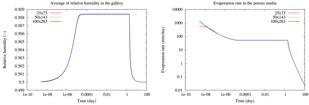
Figure 18: For each mesh and for w_{in} = 1 \text{ m}\cdot\text{s}^{-1} : average of the relative humidity in the gallery (left) and evaporation rate at the interface (right) as a function of time.
