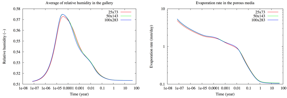
Figure 12: For each mesh and for w_{in} = 0.5 \text{ m}\cdot\text{s}^{-1} : average of the relative humidity in the gallery (left) and evaporation rate at the interface (right) as a function of time.
