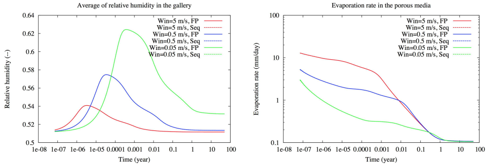
Figure 15: Comparison of the solutions obtained by the fixed-point (FP) and sequential (Seq) algorithms with the mesh 50 \times 143 : average of the relative humidity in the gallery (left), evaporation rate at the interface (right) as a function of time.
