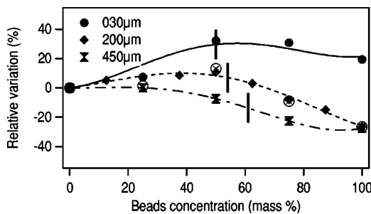
FIG. 5. Relative variation of the static friction coefficient as a function of the concentration (relative to 100- \mu m beads). 30-, 200-, and 450- \mu m beads are added to 100- \mu m beads. The crosses in open circles correspond to the case of 200- \mu m beads with sand glued at the lower surface of the plate. Vertical dashes indicate the concentration at which the mixture reaches its maximum density.
