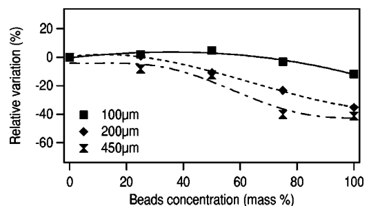
FIG. 7. Relative variation of the static friction coefficient as a function of the concentration (relative to sand). 100-, 200-, and 450- \mu m beads are added to 120- \mu m sand grains.
