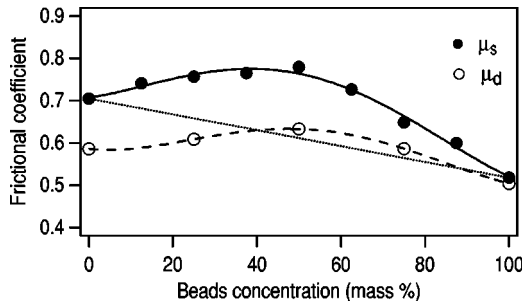
FIG. 4. Friction coefficients as functions of the mass concentration (200- \mu m beads in 100- \mu m beads).
