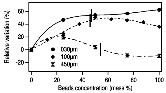
FIG. 6. Relative variation of the static friction coefficient as a function of the concentration (relative to 200- \mu m beads). 30-, 100-, and 450- \mu m beads are added to 200- \mu m beads. Vertical dashes indicate the concentration at which the mixture reaches its maximum density.
