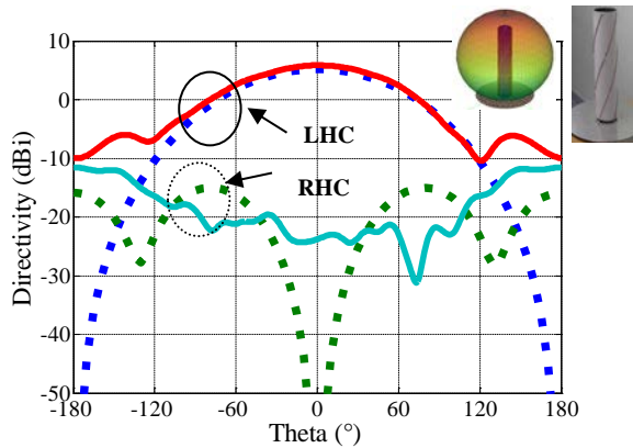
Figure 5. Experimental (continuous line) and simulated using FEKO (dashed line) results for the radiation pattern ( \Phi=0^\circ ) for the PVC-supported reference QHA1 at 120MHz. The insets give the 3D simulated radiation pattern (directivity) and the photography of the manufactured QHA1 prototype.
