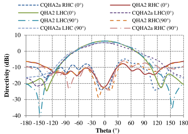
Figure 9. Measured co-polarization (LHC) and cross-polarization (RHC) components of the directivity for the references antenna QHA2 and the compact antenna CQHA2a as function of theta angle ( ^{\circ} ) for \phi=0^{\circ} (xOy) and \phi=90^{\circ} .
