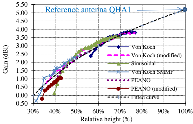
Figure 7. Gain of best-fitted CQHAs (regarding the goal function defined by Eq.(5)) as a function of the antenna relative height for various wire profiles (simulated results). The dashed curve fits all the data reported in this figure.
