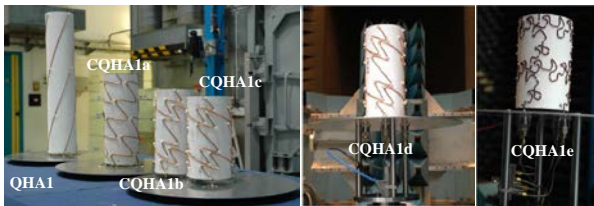
Figure 3. Manufactured wire-supported CQHAs derived from QHA1 using as shaping function various combinations of sine functions (CQHA1a, CQHA1b, CQHA1c and CQHA1d) and prefractal (Von Koch) profile combined with a sine function (CQHA1e).
