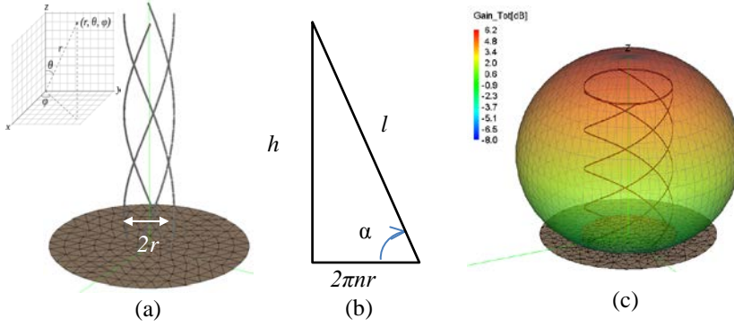
Figure 1. (a) air-supported simulation model (FEKO) for an open-end QHA including the finite-sized ground plane (the inset illustrates the adopted system of coordinates); (b) the geometrical relationship between the key descriptors of QHAs; (c) simulated (FEKO) 3D radiation pattern (gain, in dB) for a typical short-circuited QHA (axial mode).
