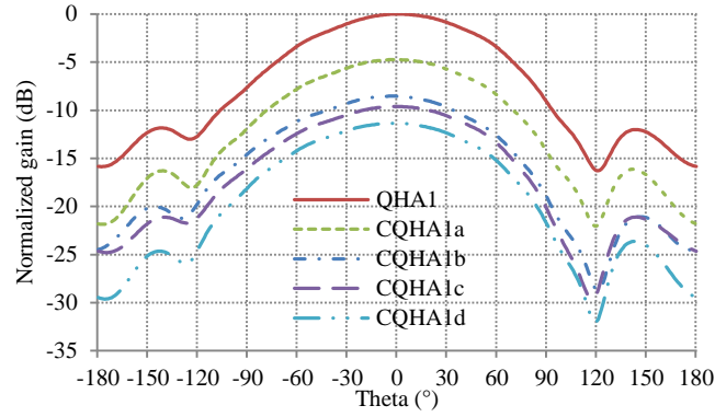
Figure 6. Measured gain of the CQHA relative to the measured gain of the QHA1 (frequency: 120 MHz).
