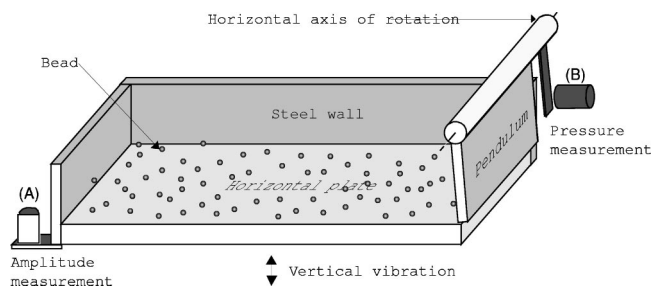
FIG. 1. Experimental setup. The experimental setup consists of a horizontal tray that oscillates sinusoidally along the vertical. The vertical displacement of the tray is measured with the help of an inductive sensor (A). Three of the sidewalls are attached to the horizontal plate, whereas the last one (the pendulum, on the right-hand side) rotates freely around a horizontal axis, which is fixed in the laboratory frame. The angle that the pendulum makes with the vertical direction is measured with the help of a second inductive sensor (B).
