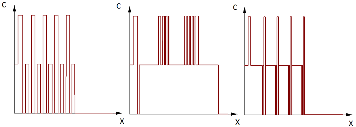
Figure 3: Distributions of differentiated cells as a function of the space variable for three different sets of parameters: q_1 = q_2 = 0.01 (left), q_1 = q_2 = 0.01 , D_2 = 0.5 (middle), q_1 = 0.1 , q_2 = 0.01 (right). The value c = 0 corresponds to c_A = 1, c_1 = 0, c_2 = 0 ; c = 1 to c_A = 0, c_1 = 1, c_2 = 0 and c = 2 to c_A = 0, c_1 = 0, c_2 = 1 .
