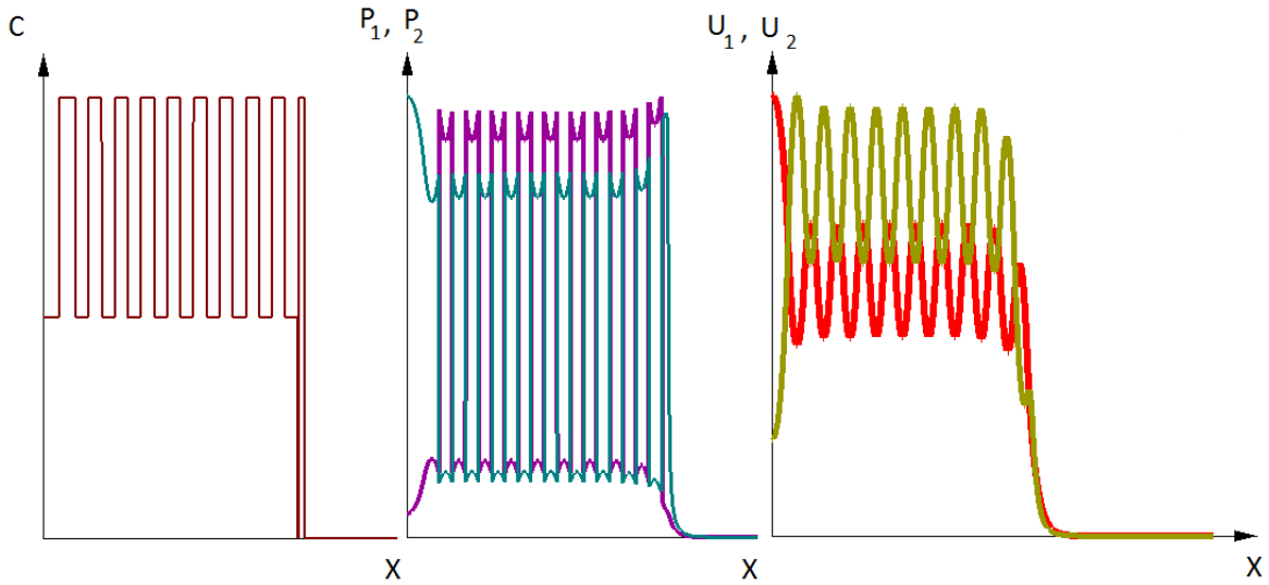
Figure 2: A snapshot of solution. The curves show the values of the corresponding concentrations as functions of the space variable x . A travelling wave of cell differentiation propagates from the left to the right. The distribution of cells B_1 ( c = 1 ) and B_2 ( c = 2 ) behind the wave is periodic (left image). Distributions of p_1, p_2 (middle) and of u_1, u_2 (right) oscillate in space. The value c = 0 corresponds to c_A = 1, c_1 = 0, c_2 = 0 ; c = 1 to c_A = 0, c_1 = 1, c_2 = 0 and c = 2 to c_A = 0, c_1 = 0, c_2 = 1 . (see the explanation in the text).
