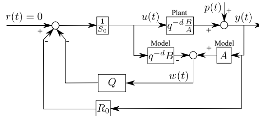
Fig. 7.3 The Youla–Kučera parametrized RS digital controller.
