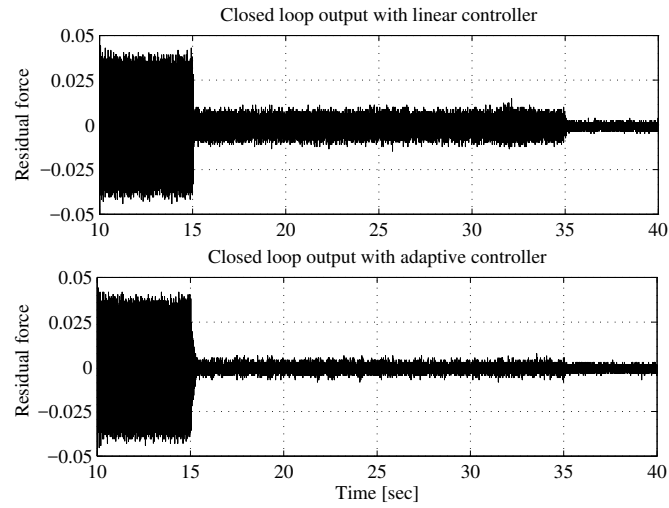
Fig. 12.4 Residual force in closed-loop with linear robust controller (upper plot) and with adaptive controller (lower plot). The experiments are started in open-loop for 5 sec and the disturbances are removed at t=35 sec. Range of frequency variation: \pm 2.5 Hz.
