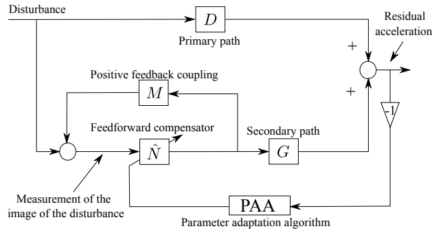
Fig. 4.2 Adaptive feedforward disturbance compensation.
