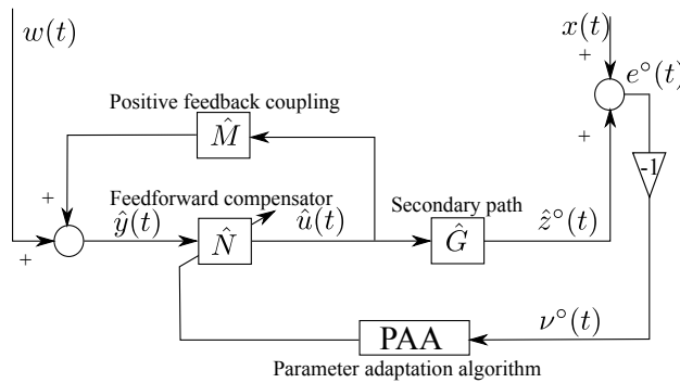
Fig. 14.8 Estimation of the feedforward compensator using a simulated adaptive feedforward compensation scheme in self-tuning regime.
