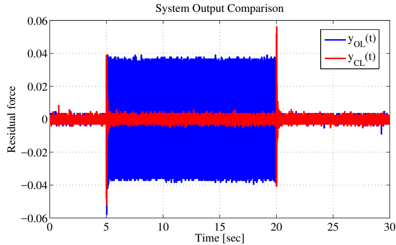
Fig. 8.7 Time response results for 70 Hz disturbance in open-loop and in closed-loop with the redesigned controller.
