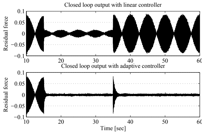
Fig. 12.10 Residual force with step frequency changes (+5 Hz) in closed-loop with linear controller (upper plot) and with adaptive controller (lower plot). In both cases, the system is in open-loop until t=15 sec.
