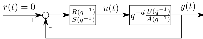
Fig. 7.1 Discrete feedback RS controller.
