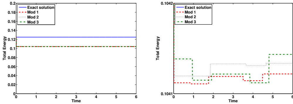
Figure 4: Comparison of the energy associated with analytical solution and the energy associated with approximate solutions for some modified mass matrices with Crank-Nicolson method ( \Delta x = \frac{1}{6} and \Delta t = \frac{1}{100} ). The figure on the right hand side represents a zoom of the figure on the left hand side.
