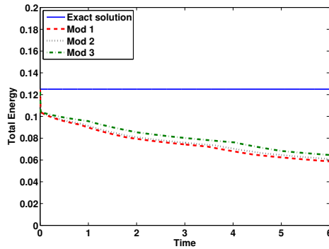
Figure 6: Comparison of energy associated with analytical solution and energy associated with approximate solutions for modified mass matrices with backward Euler method ( \Delta x = \frac{1}{6} and \Delta t = \frac{1}{100} ).
