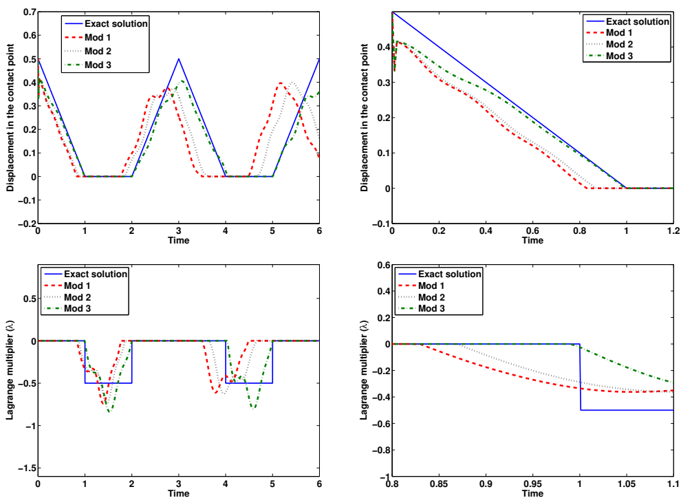
Figure 7: Comparison of analytical (u, \lambda) and approximate (U_h^n, \lambda^n) solutions for some modified mass matrices in the contact node with Paoli-Schatzman method ( \Delta x = \frac{1}{6} and \Delta t = \frac{1}{100} ).
