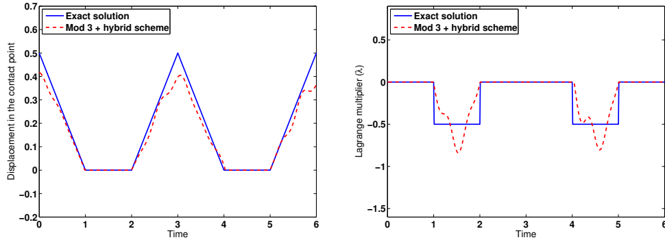
Figure 9: Comparison of analytical (u, \lambda) and approximate (U_h^n, \lambda^n) solutions for the modified mass matrix (Mod 3), in the contact node with hybrid scheme (\Delta x = \frac{1}{6} and \Delta t = \frac{1}{100}) .
