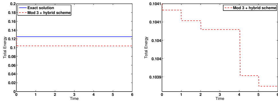
Figure 10: Comparison of the energy associated with analytical solution and the energy associated with approximate solutions for the modified mass matrix (Mod 3) with hybrid scheme (\Delta x = \frac{1}{6} and \Delta t = \frac{1}{100}) . The figure on the right hand side represents a zoom of the figure on the left hand side.
