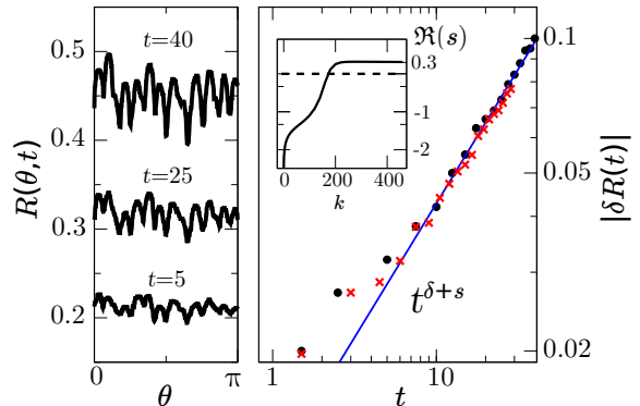
FIG. 3: Left: Shock radius by angular sector R(\theta, t) at successive times (see [30] for its definition). The line thickness represents the mean free path in the shock front, or about half its average width w \approx 0.01 . Right: Corrugation width \delta R \sim t^{\delta+s} with theoretical exponent s \simeq 0.3 (solid line) and numerical validation for \alpha = 0.3 (circles) and \alpha = 0.8 (crosses). Inset: Real part of the dispersion relation s(k) for the unstable mode, crossing the marginal stability line \Re(s) = 0 (dashed line), with a plateau at \Re(s) \approx 0.3 .
