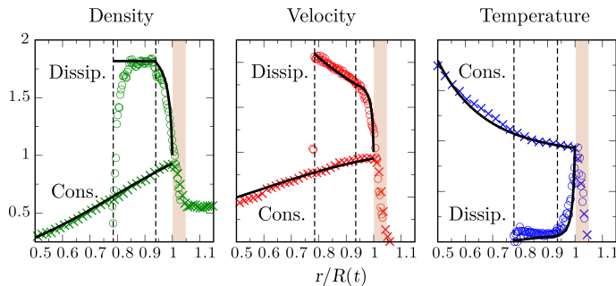
FIG. 2: Hydrodynamic profiles from MD simulations for dense conservative (crosses) and dissipative (circles) fluids with \phi_{rest} = 0.3 , and analytical solutions (solid lines). Profiles are rescaled by the Rankine-Hugoniot boundary value (see [30]), from left to right: n(\lambda)/n_{RH} , u(\lambda)/u_{RH} and \Theta(\lambda)/\Theta_{RH} with \lambda = r/R(t) . The conservative solution is partitioned into the gas at rest, the shock front (shaded area) and the self-similar bulk. This is the first validation of a TvNS-like solution in a dense fluid. For any dissipation i.e. \alpha < 1 (here \alpha = 0.8 ), the bulk structure becomes threefold, as shown by dashed vertical lines: the cooling region between the front and R_c \approx 0.93R ; the maximally dense cold fluid down to R_i \approx 0.78R ; and the central cavity.
