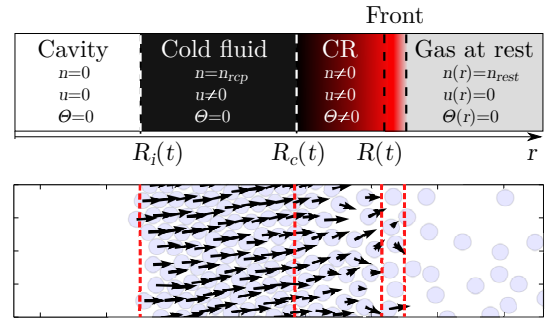
FIG. 1: Section of the blastwave: cartoon (top) and hard sphere MD simulation (bottom). Dissipation causes particles to accrete into a dense, hollow shell. Eqs.(5)-(7) reveal its layered structure. First, the shock front where particles from the blast collide and mix with those at rest, creating incoherent motion. Then, a fixed-width cooling region (CR) where further compression occurs as temperature is dissipated, and finally a self-similar cold fluid region where velocities are well aligned, around a central cavity. This stands in stark contrast with the elastic case, where the bulk of the blast is comprised of a single, entirely self-similar region.
