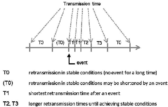
Fig. 2. GOOSE transmission
