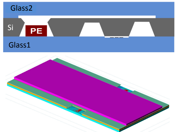
Figure 9. HDPE filling and Glass2 bonding
