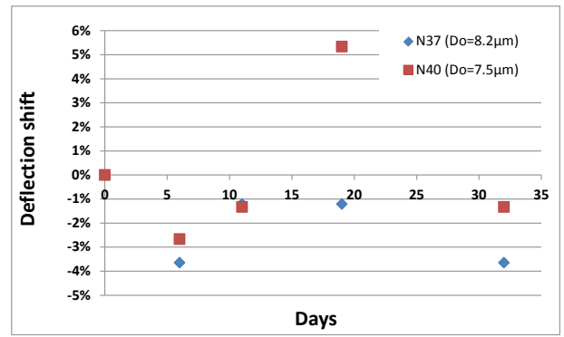
Figure 4. Membrane deflection shift versus time after nuclear irradiation Do denotes the deflection at initial time
