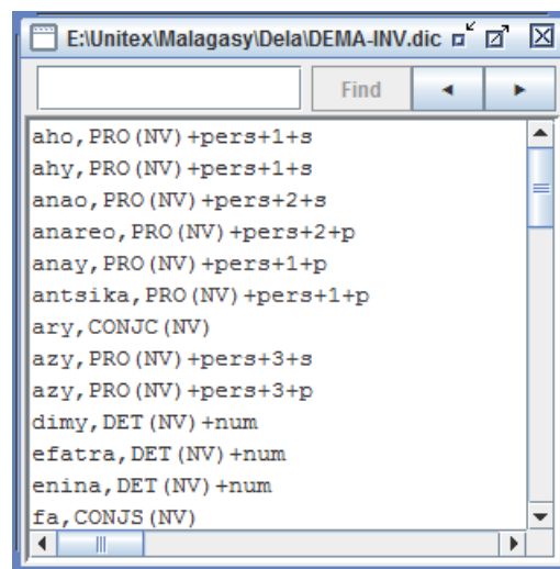
Fig. 7: Excerpt of a dictionary of invariable words
