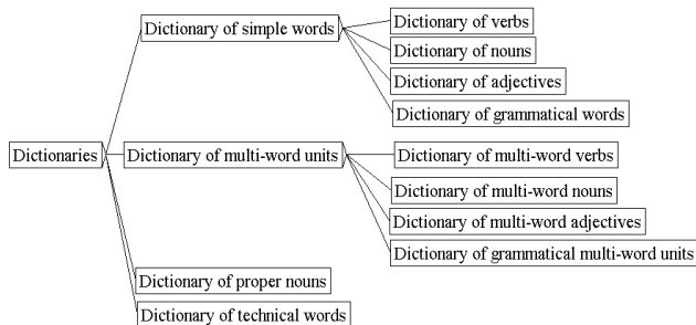
Fig. 2: Structure of a Malagasy NLP dictionary
