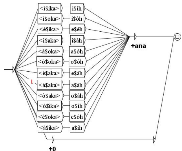
Fig. 4: Transducer of generation of allomorphs N1av
