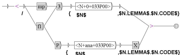
Fig. 5: Transducer of combination of morphemes 033P00
