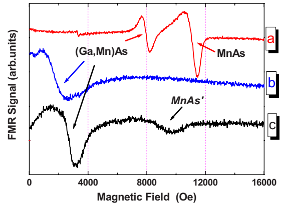
FIG. 3. (Color online) FMR spectra at T=4 K for H \parallel [001] (a), H \parallel [1-10] (b), and H \parallel [110] (c) of the MnAs/(Ga,Mn)As bilayer. The low intensity MnAs spectrum in (c) results from a fraction of the MnAs layer with a different orientation as compared to the main A phase, characterized by an in-plane intermediate axis.
