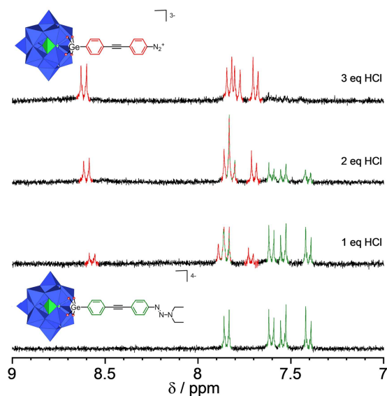
Figure 1. ^1\text{H} NMR monitoring of the formation of the diazonium-derived hybrid \mathbf{K}_{\text{Ge}}[\text{N}_2^+] from \mathbf{K}_{\text{Ge}}[\text{N}_3\text{Et}_2]
