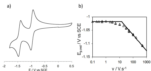
Figure 2. a) Cyclic voltammetry at a glassy carbon electrode (2 mm diameter) of \text{K}_{\text{Ge}}[\text{I}] (1 mM) in a 0.1 M TBAPF 6 MeCN solution at the scan rate \nu = 0.1 \text{ V}\cdot\text{s}^{-1} ; b) 1 st reduction peak potential variation with \nu . Symbols: experimental values, lines: predicted variations, see text.
