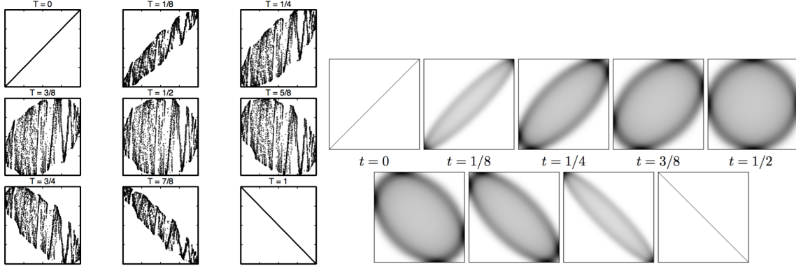
Figure 6: Relaxed Euler boundary value problem on X = [0, 1] with boundary conditions s_* = \text{Id} , s^* = -\text{Id} . The solution for this particular instance is unique and known [BFS09], it involves non-deterministic generalized flows see §2.3. Horizontal axis: initial particle position x \in [0, 1] . Vertical axis: particle position in [0, 1] at some specified time t . Left: discretization based on permutations [Bre08] see (18). Right: convex relaxation as multi-marginal problem [BCC + 15], regularized via entropy penalization, see (23).
