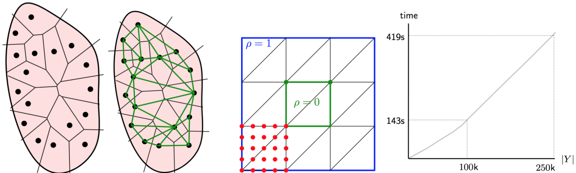
Figure 4: Left: Laguerre cells and their dual graph. Center: Numerical test case setup. Right: Computation time versus number of Dirac masses.
