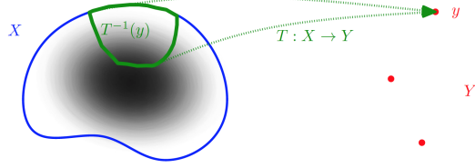
Figure 1: A map T sends domain X (blue boundary), equipped with a density \mu = \rho \text{Leb}_X (grayscale) onto a finite set Y (red dots). The push-forward \nu = T_{\#}\mu is defined by \nu(\{y\}) = \mu(T^{-1}(\{y\})) (mass of the green region), for all y \in Y .
