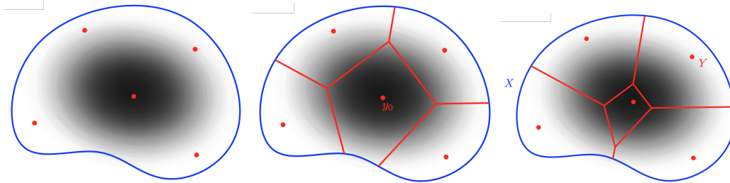
Figure 3: Left: Domain X (blue boundary), population density \rho (grayscale), and bakeries Y (red dots). Center: Voronoi regions (red boundaries) attached to the bakeries. Right: Laguerre diagram, depending on both the bakeries positions Y and their prices \psi : Y \rightarrow \mathbb{R} .
