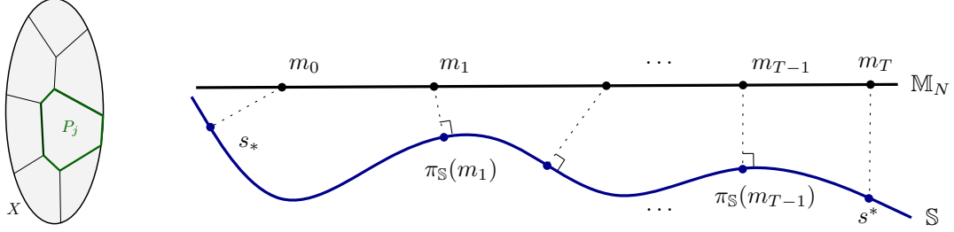
Figure 7: Left: partition \mathcal{P}_N of the domain X into N regions. Right: illustration of the discretization (28). The maps (m_t)_{t=0}^T belong to a linear subspace \mathbb{M}_N (black) of L^2(X) , whereas \pi_S(m_t) denotes their projection onto the manifold \mathbb{S} (blue).
