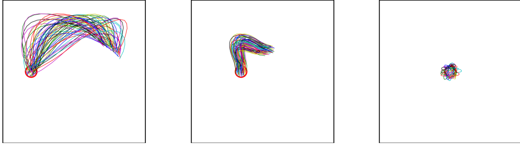
Figure 9: Particles trajectories in the case t_{\max} = 1.5 , see Figure 8. Left: trajectories originating from inside this red circle seem strongly non-deterministic. Center: trajectories originating from this circle remain grouped. Right: particles around the domain center move little.
