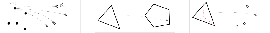
Figure 2: The three paradigms of numerical optimal transport. I: Fully discrete, II: Fully continuous, III: Semi-Discrete. All illustrations of this section courtesy of Q. Merigot.
