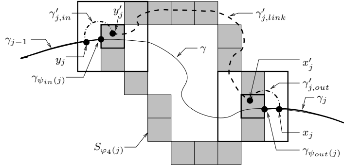
FIGURE 3. Construction of the path \gamma' - step 2.
