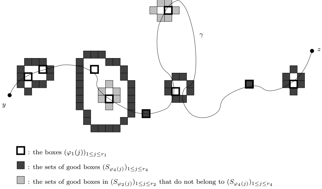
FIGURE 2. Construction of the path \gamma' - step 1.
