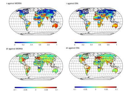
Fig. 3: Correlations of the updated C-band LPRM against MERRA-Land and ERA-Land
