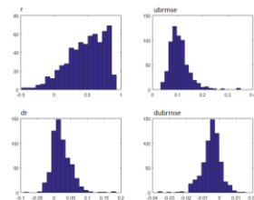
Fig. 4: Histograms of the comparison between C-band AMSRE LPRM and all the available ground observations from the international soil moisture network.
