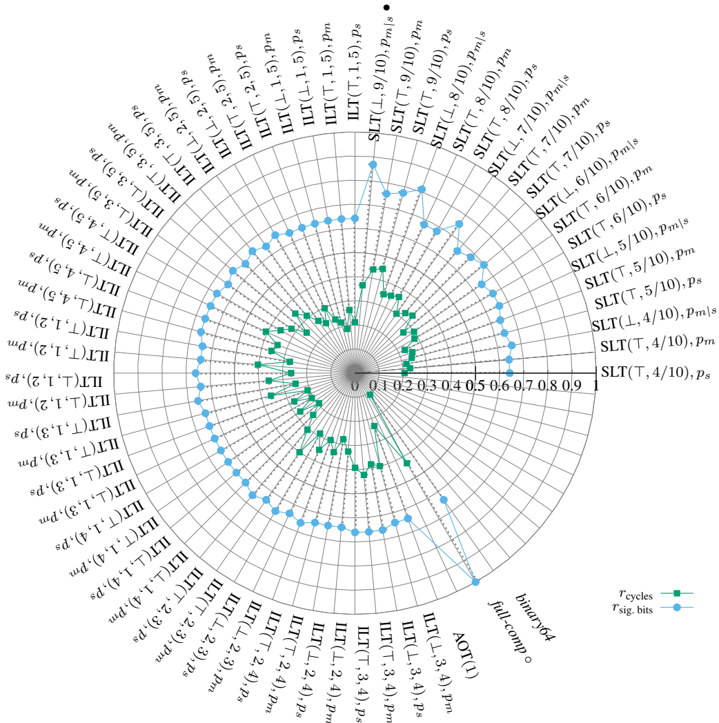
Figure 10. Results exploration in the case of HORNER's algorithm with data x_3 ( r_{cycles} closer to 0 the better, r_{sig.bits} closer to 1 the better), \circ denotes the program returned with R_{acc} , and \bullet the one returned with R_{exe} .
