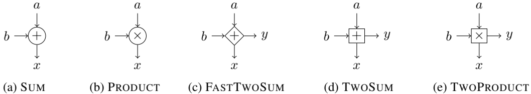
Figure 2. Diagrams for basic floating-point operations (a), (b) and EFT algorithms (c), (d), and (e).
