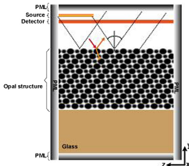
Figure 2. Representation of the computation cell used in FDTD calculations.
