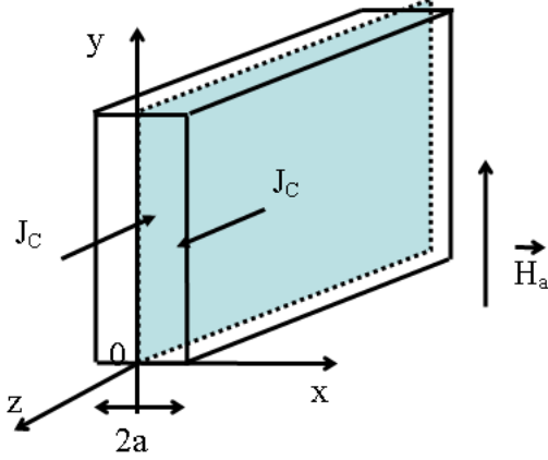
Fig. 2: A symetric distribution of current density in a superconducting plate.
