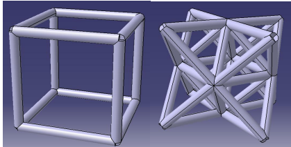
Figure 5. ELEMENTARY CUBIC, OCTET TRUSS AND HEXAGONAL LATTICE STRUCTURE
