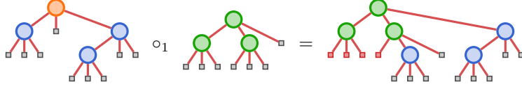
FIGURE 5. Interpretation of the partial composition map of the ns operad \text{FCat}^{(2)} in terms of 2-leafy trees.
