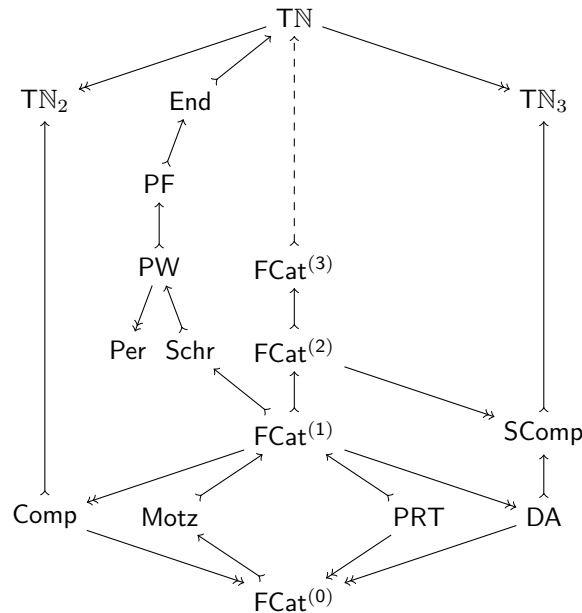
FIGURE 1. The diagram of ns suboperads and quotients of \mathbb{T}\mathbb{N} . Arrows \rightsquigarrow (resp. \rightarrow ) are injective (resp. surjective) ns operad morphisms.
