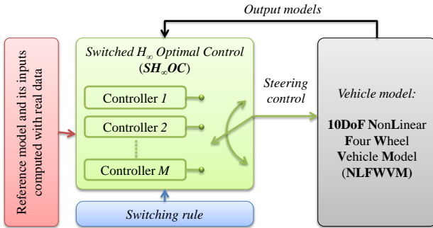
Fig. 2. A diagram block of switched H_\infty optimal control coupled reference model and nonlinear vehicle model
