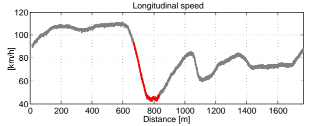
Fig. 4. Measured longitudinal speed and braking action between the positions 650 m and 850 m
