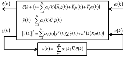
Fig. 1. Switched H_\infty State Feedback Optimal Control
