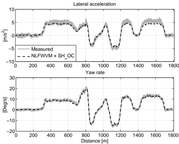
Fig. 5. lateral acceleration and yaw rate: measurements and those computed by L2WVM + SH_\infty OC and NLFWVM + SH_\infty OC
