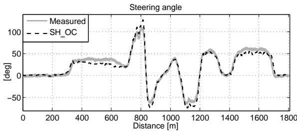
Fig. 6. Steering angle: Measured and those computed by SH_\infty OC + NLFWVM
