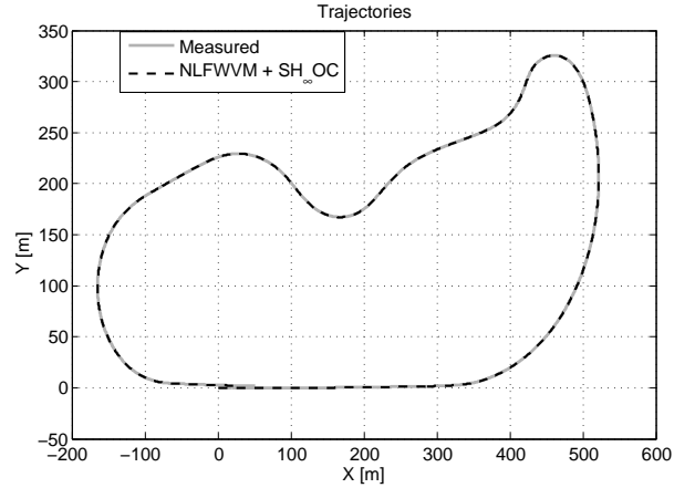
Fig. 7. Trajectories: Reference and those of NLFWVM + SH_\infty OC
