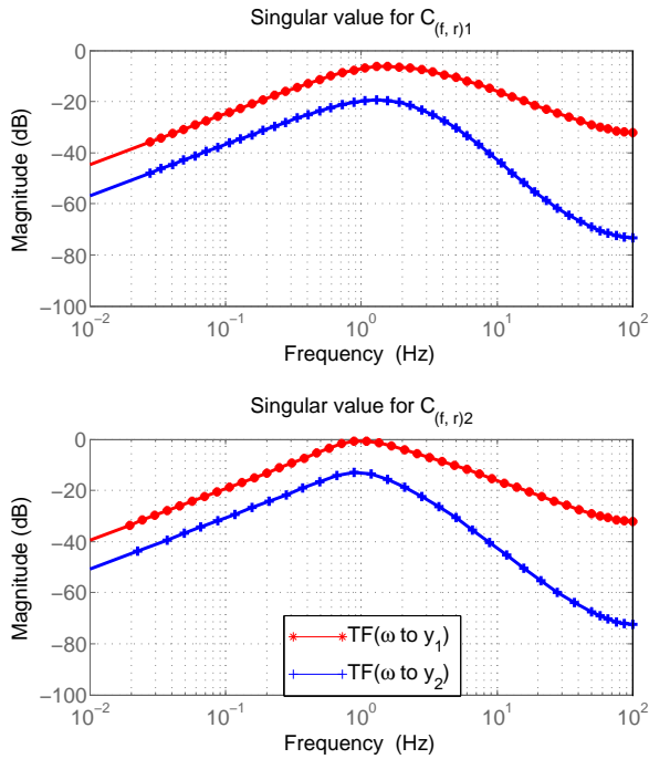
Fig. 9. Transfer function of system ((\bar{A}_i - \bar{B}_i \bar{K}_i), \bar{F}_i, \bar{C}_i) for two values of cornering stiffnesses C_{(f,r)1} and C_{(f,r)2} coefficients, between \omega to \dot{y}
