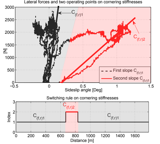
Fig. 3. Experimental lateral tire force characteristic, switching rule on cornering stiffnesses and two operating points C_{(f,r)1} and C_{(f,r)2}
