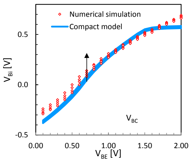
Figure 4. Graphene Fermi potential versus V_{BE} curves for different V_{CB} (2, 3, 4, 5 V), numerical simulation and compact model simulation.
