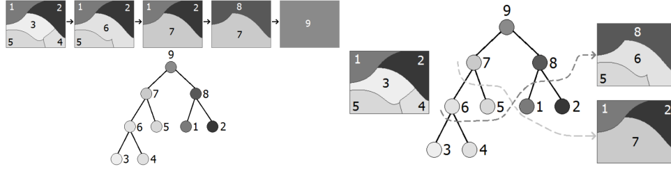
Figure 4 An example of the construction of a BPT (left). Starting from an initial partition (the leaves, here nodes 1 to 5), the most similar regions are merged, creating a new node in the tree, and a new partition. This process is iterated until only one region remains (the root of the tree). Two possible prunings of the BPT (right). We can only select nodes that form a partition of the initial image.
