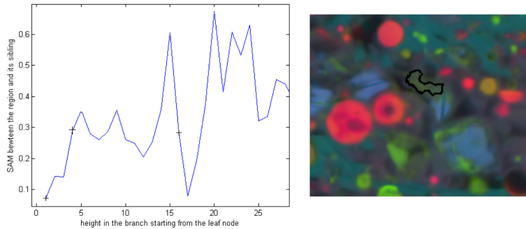
Figure 11 Evolution of SAM between nodes at a certain height in a branch and their siblings, and the region kept in the branch with the chosen pruning strategy, using a threshold on SAM of 0.15rad and a threshold on size of 10 pixels. On the graph, the black crosses indicate (from left to right) either the leaf node, the node kept by the proposed pruning strategy or the node kept considering only the size.
