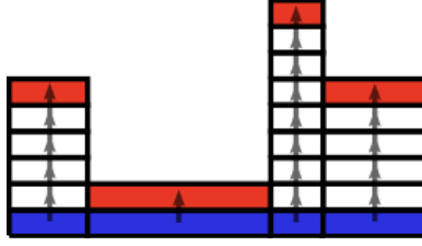
FIGURE 1. A Kakutani–Rokhlin partition
